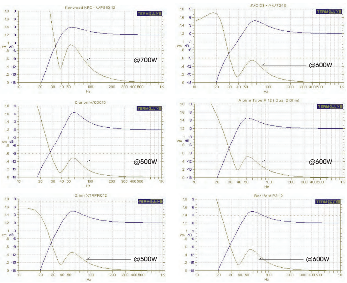
Response chart based on 3.7L driver displacement, For general guidance only.
