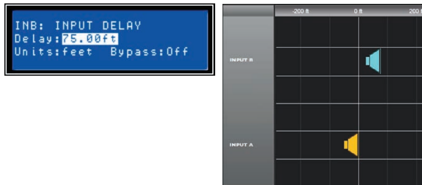
Illustration 5.1: Input B Delay is set to 75 feet. In this illustration, speaker array B is said to be 75 feet in front of Main speaker array A. The effect of air temperature is also automatically calculated for the total delay time using the Temperature value entered in the Setup Menu.
