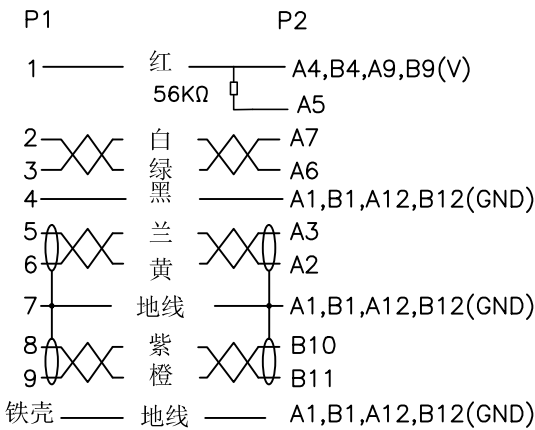
PIN OUT
