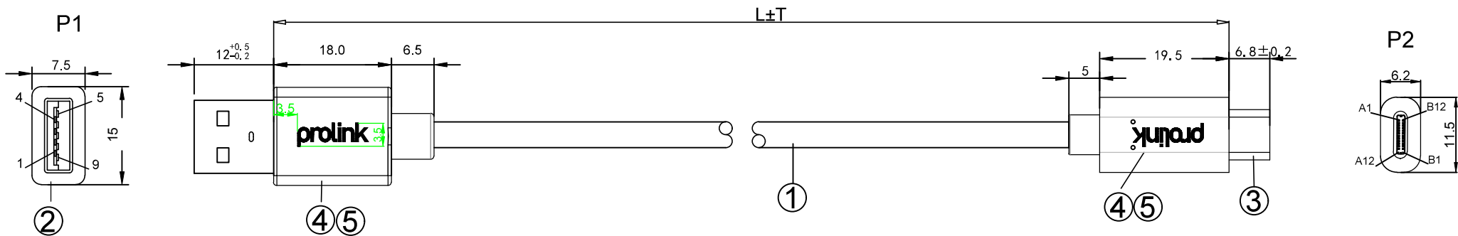
P/N CHART
