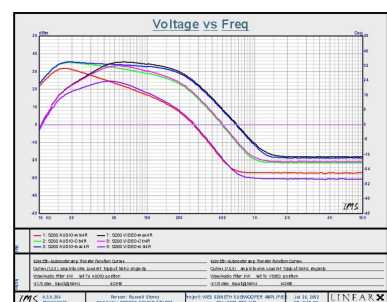
Graph showing Gain and Freq Control settings
