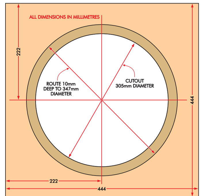
EXTERIOR FRONT PANEL (FRONT VIEW)
