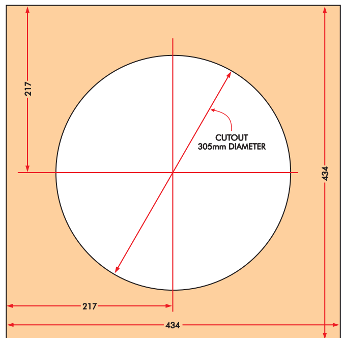
INTERIOR FRONT PANEL
