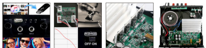
2x front microphone inputs with level and echo | RIAA Phono pre-amplifier to support turntable input | Class AB amplifier stage | Toroidal power transformer
