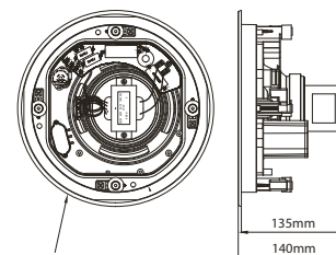
With grille: Ø257mm Without grille: Ø247mm Hole Cut: Ø220mm
