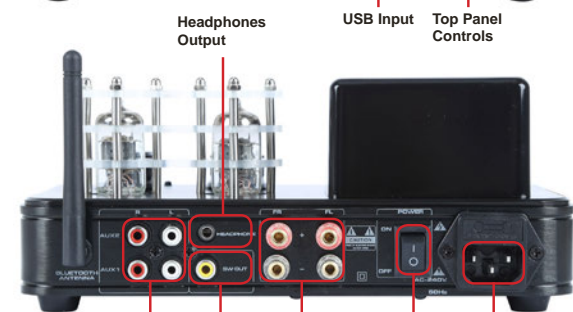
AUX1 / Subwoofer AUX2 Output Speaker Outputs Power Switch AC Power Cord
