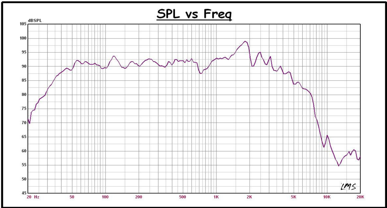
FIG. 1: FREQUENCY VS.SPL
