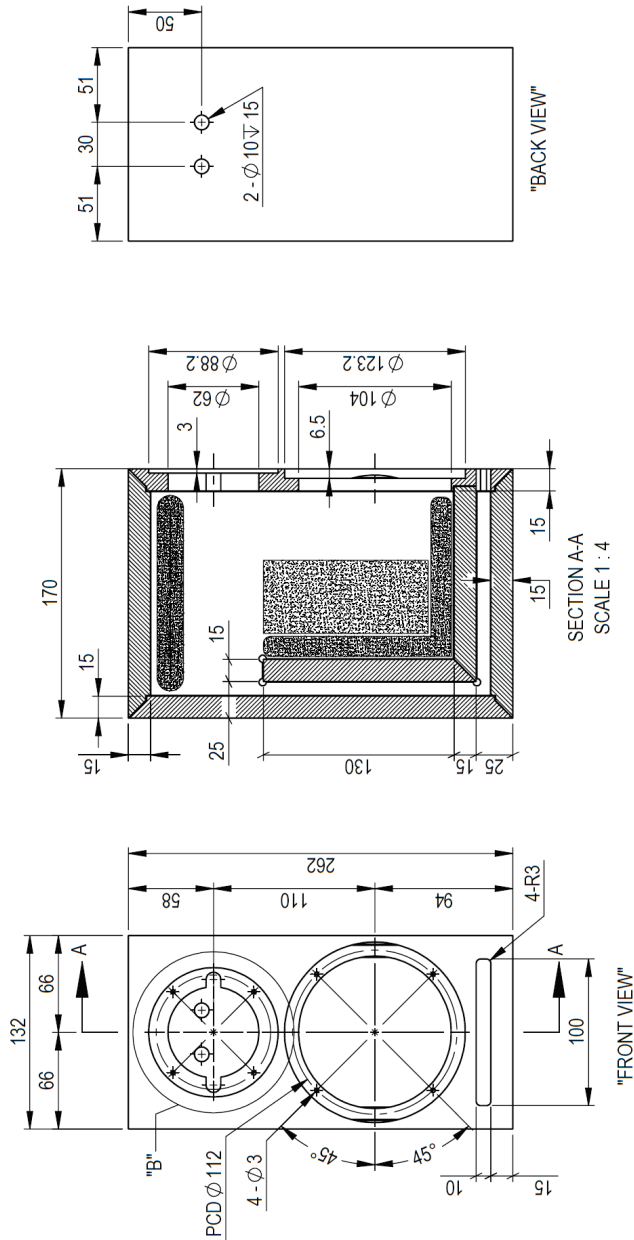
Mechanical drawing (size in mm) / Micro-C
