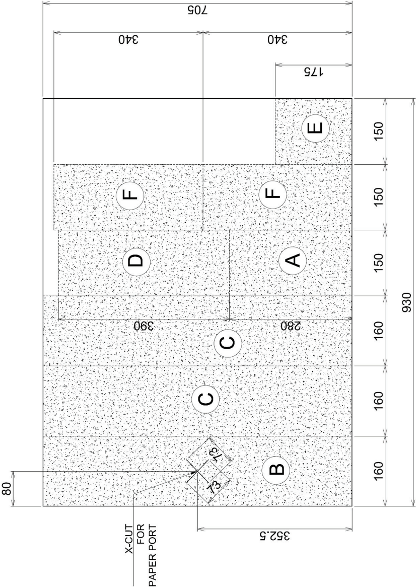
Damping Material Cut Pattern (Size in mm)
