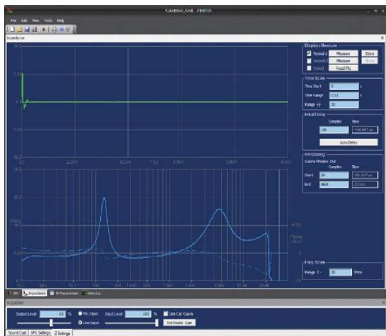
FIGURE 3: FINE SPL impedance magnitude and phase graph.
