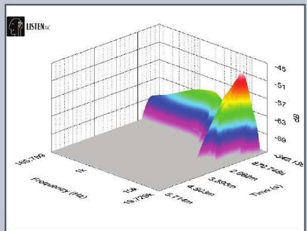
FIGURE 15: Scan-Speak 18WU4747T00 SoundCheck Wigner-Ville plot.
