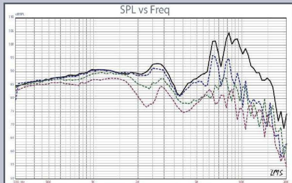
FIGURE 11: Scan-Speak 18WU4747T00 on- and off-axis frequency response.
