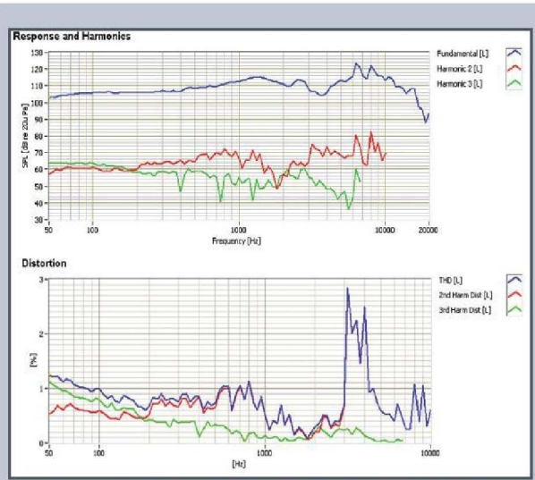
FIGURE 13: Scan-Speak 18WU4747T00 SoundCheck distortion plot.
