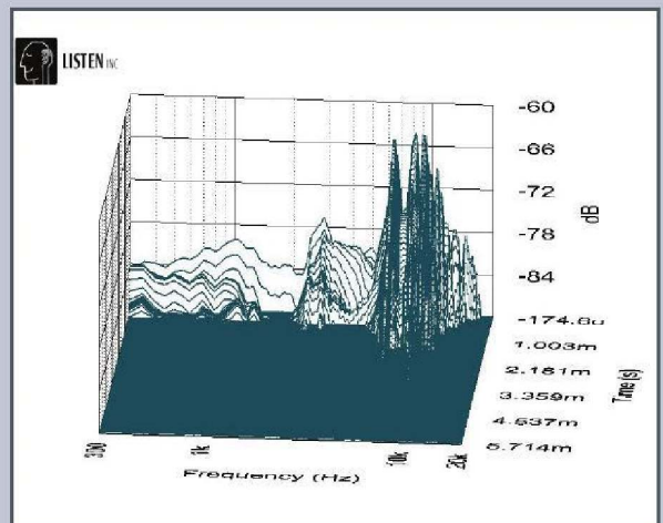
FIGURE 14: Scan-Speak 18WU4747T00 SoundCheck CSD waterfall plot.
