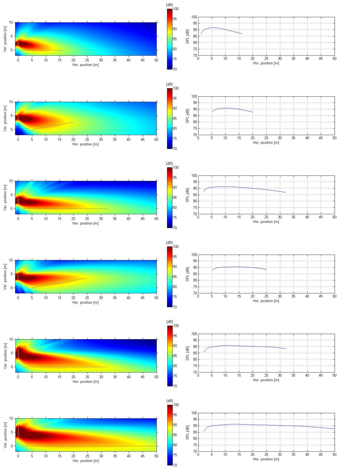
Examples of vertical beam cross sections and SPL at ear level (2 x VARI-B, 2 x VARI-B+E, 2 x VARI-B+E+E)
