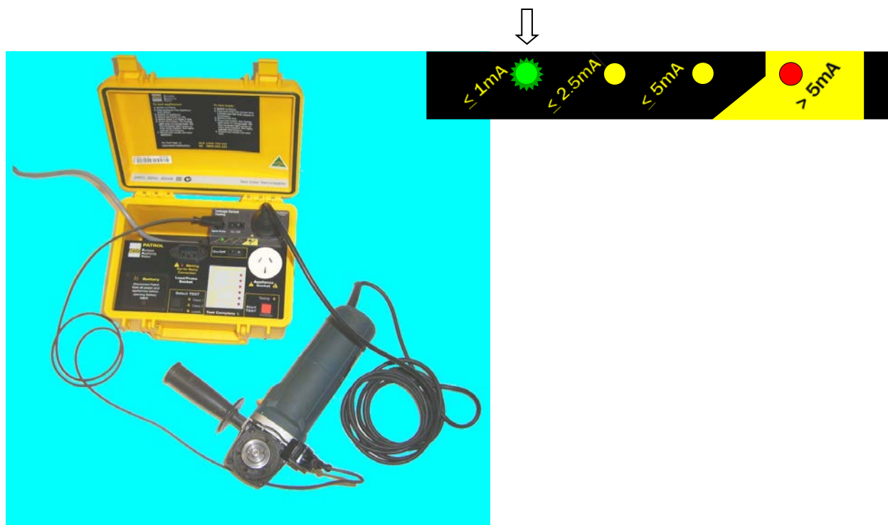
Figure 4.5.2-1 Class II Appliance Pass.
