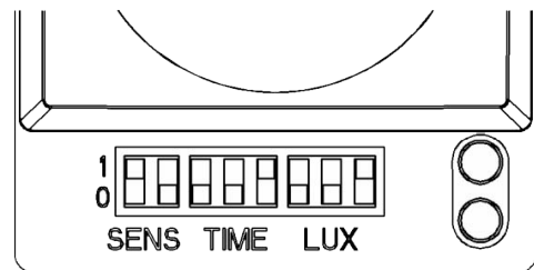
Dipswitches control motion & daylight sensitivity and on-time delay.
