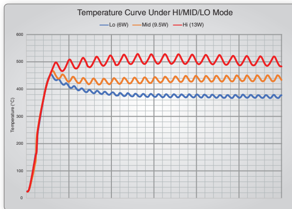
Solder Master maintains consistent tip temperature for hassle free soldering in both indoor and outdoor environments.
