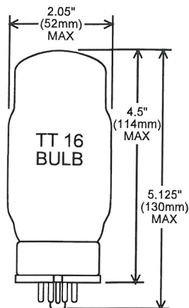
GLASS BULB LARGE WAFER OCTAL WITH BARRIERS 7 PIN LOW LOSS B7-99
