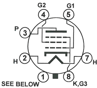
BOTTOM VIEW BASING DIAGRAM JEDEC 7AC PIN 1 - NO CONNECTION OR BASE SHELL
