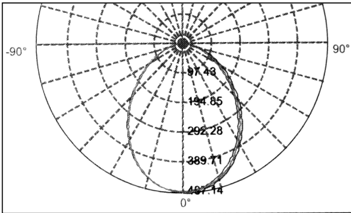
Light Distribution Curve
