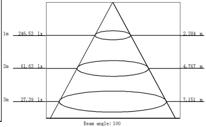
Lux-Distance Curve
