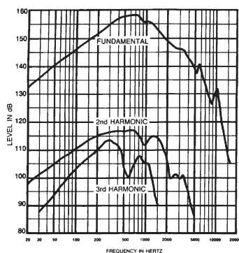
Figure 1. Distortion Response - Plane Wave Tube (1", 6-Watt Input)
