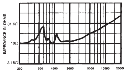
Figure 4. Impedance Response - EC100 Horn
