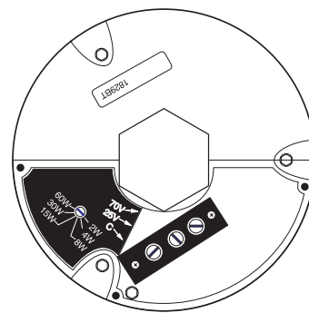
Figure 5. Driver - Rear View
