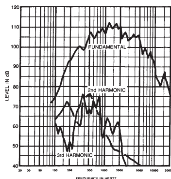
Figure 2. Distortion Response - EC100 Horn
