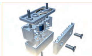
Clip fixation using Easy-Rope, Easy-Ring and Easy-Stop
