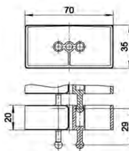
Desk to Channel Kit
