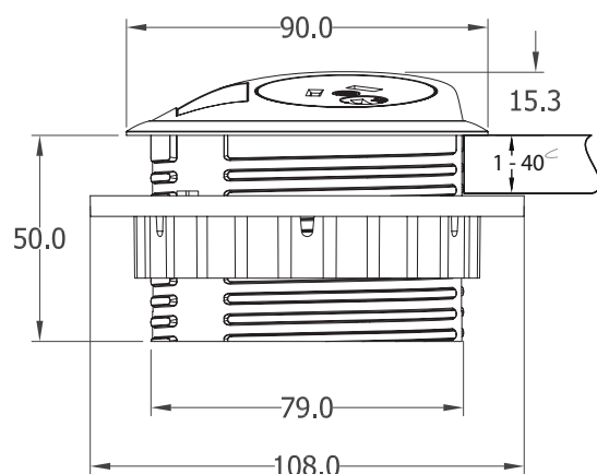
TUF A+C Charger
