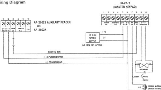
Dual-Station Access Control Door Lock
