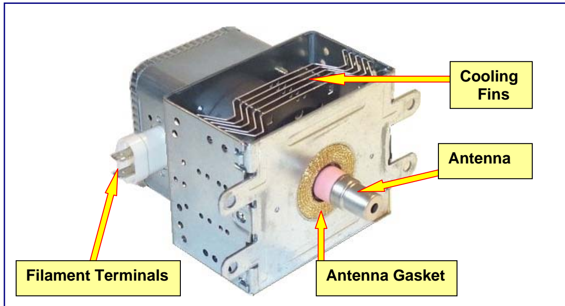
Magnetron components
