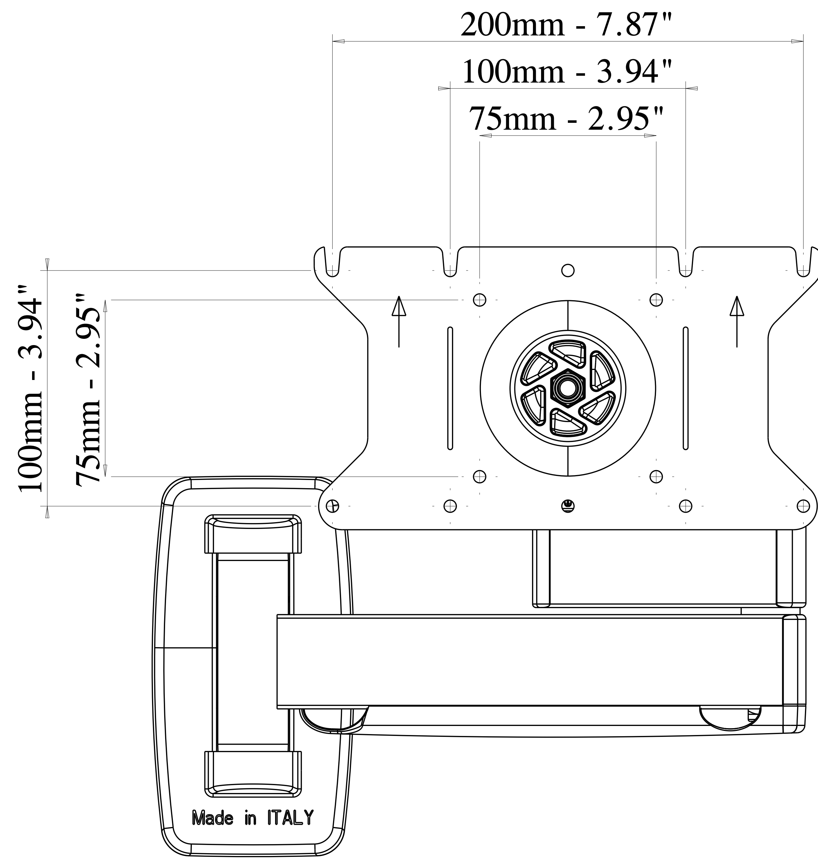
VISTA FRONTALE - FRONT VIEW
