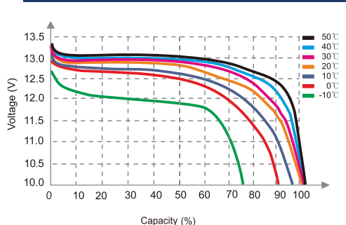
Different Temperature Discharge Curve(0.2C)
