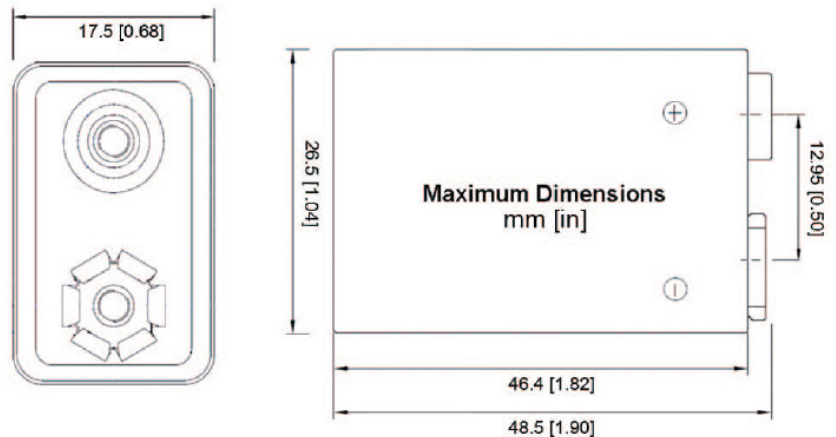
Figure 1: U9VL-J-P Dimensions
