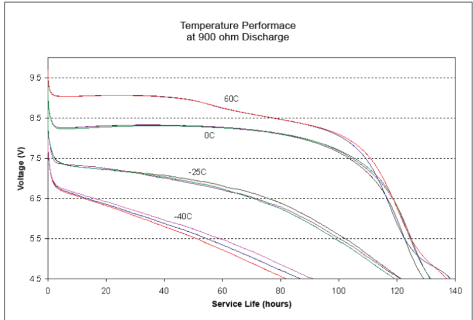
Figure 5: 900 Ohm Discharge at Various Temperatures
