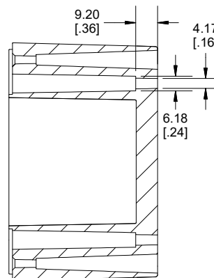
SECTION C-C MOUNTING HOLE
